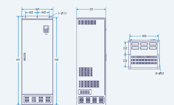
355-500kW Floor mounting Installation diagram
