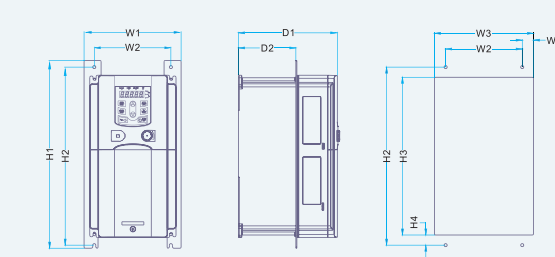
11-15kW Flange mounting installation diagram
