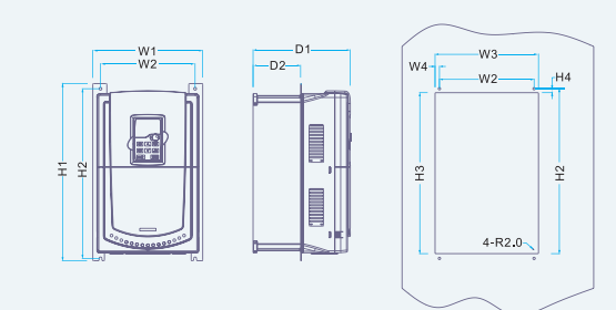
11-15kW Flange mounting installation diagram
