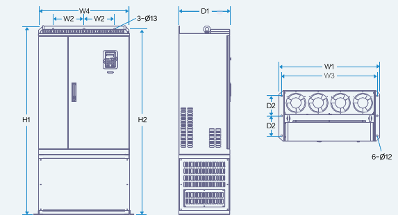
355-500kW Floor mounting Installation diagram
