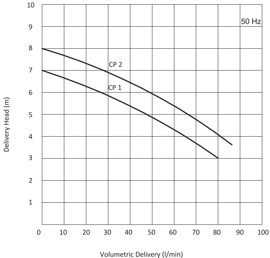
Performance Curve
