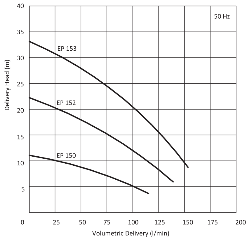
Performance Curve
