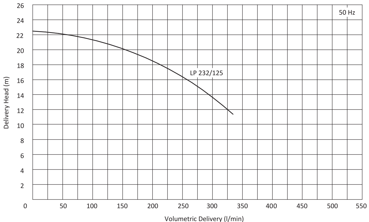
Performance Curve
