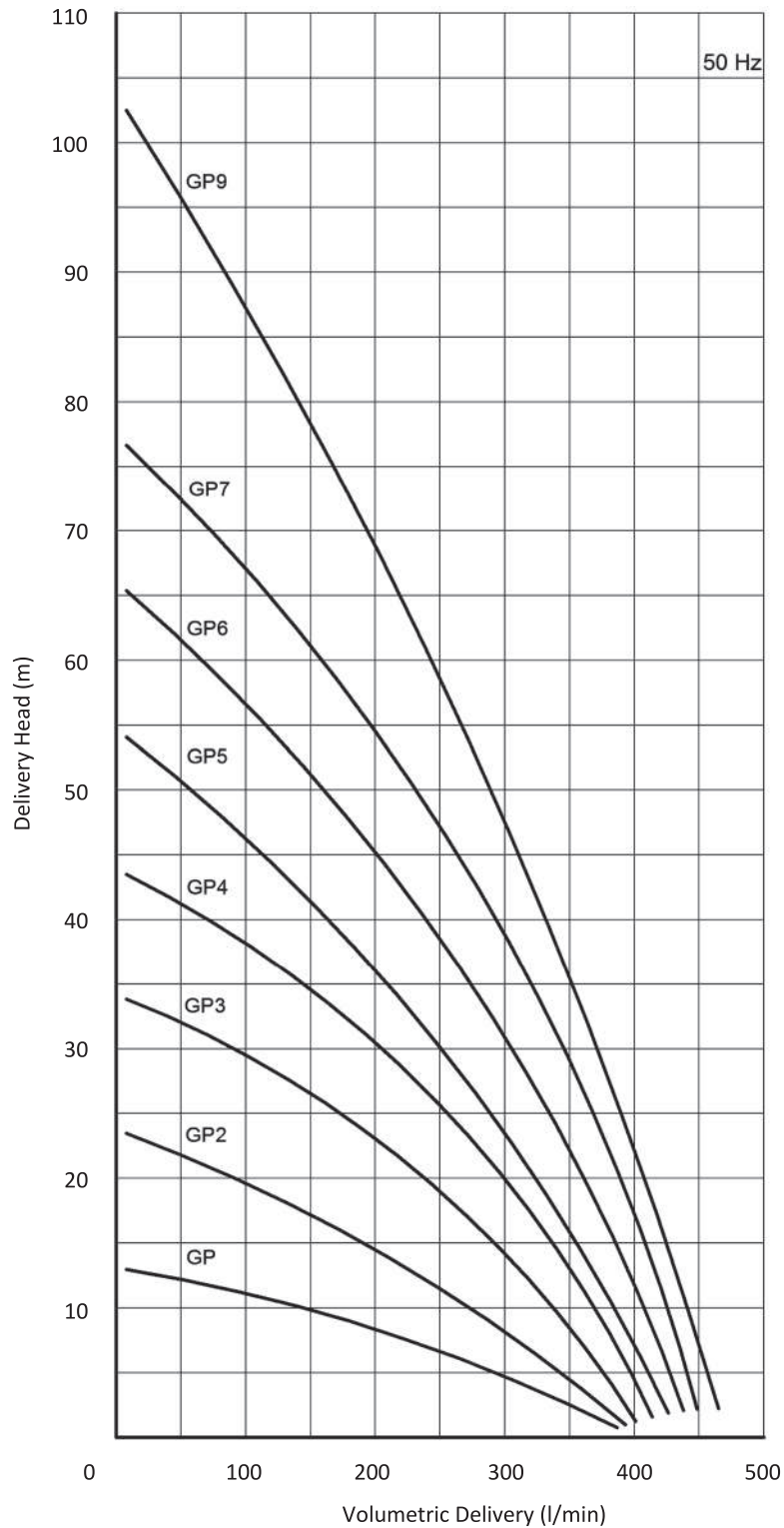
Performance Curve
