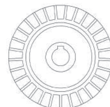
Figure 4 - Peripheral impeller of FP90 pump
