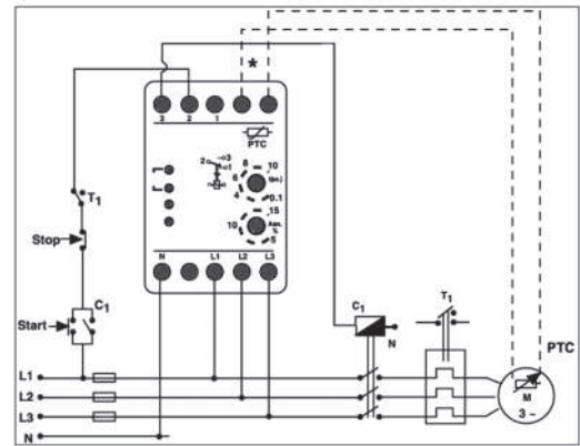
Figure 20 - Thermistor - relay connection
