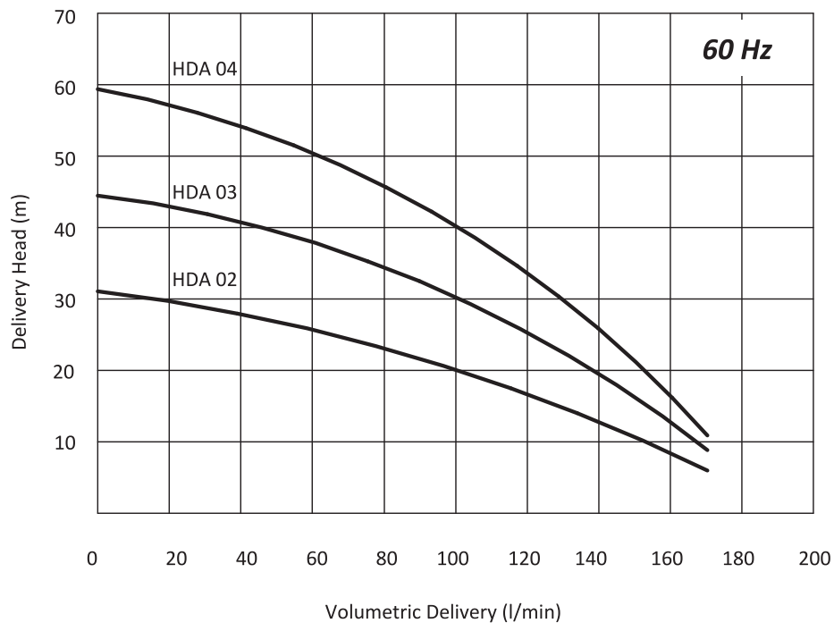
Performance Curve
